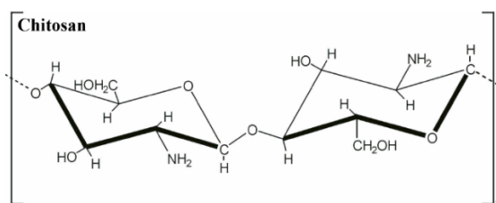
Figure 1. Structural formula of Chitosan ( https://www.researchgate.net/figure/Chemical-structure-of-chitosan_fig4_355787682 )
