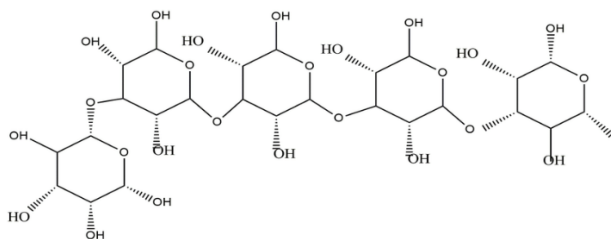
Figure 2. Structural formula of (1,3)- \beta -Glucans
