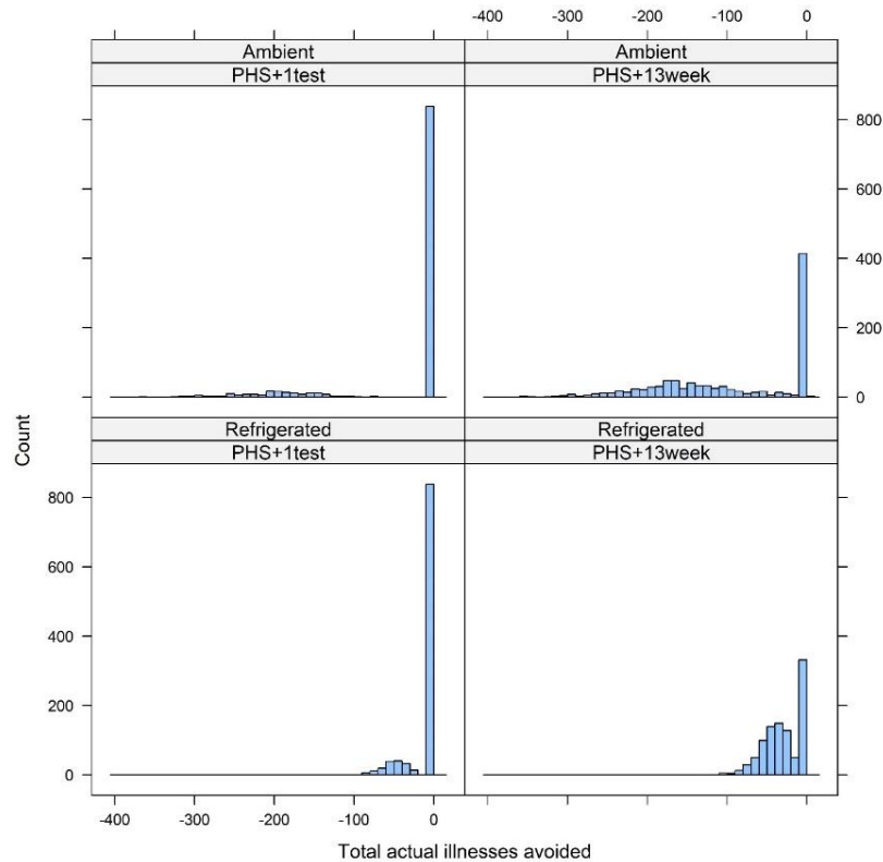
Figure 16: Histogram of illnesses avoided for a medium sized farm over 1,000 model iterations by supply chain temperature and detection method: PHS and 1 test per production cycle or PHS with regular 13 week tests.
