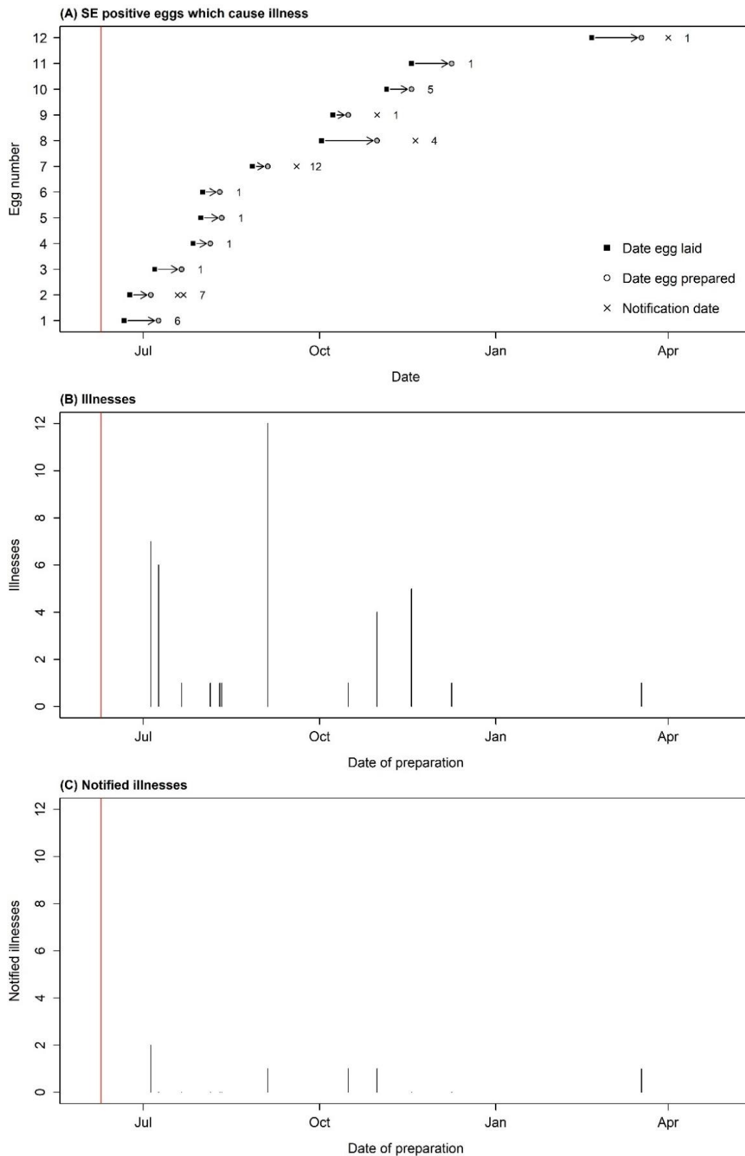
Figure 10: Small Farm with refrigeration iteration #1: (A) individual SE-positive eggs which caused illness, (B) number of illnesses and (C) number of notified illnesses. The red solid line is the date the farm started producing SE-positive eggs. The black squares represent the date each egg was laid; the circles indicate the date the egg was prepared and consumed. The length of the arrow is the actual shelf-life of the egg; longer arrows indicate longer times. The crosses represent when notified cases were reported after visiting a doctor and providing a stool sample, and the number indicates the total number of cases of illness caused by that egg.
