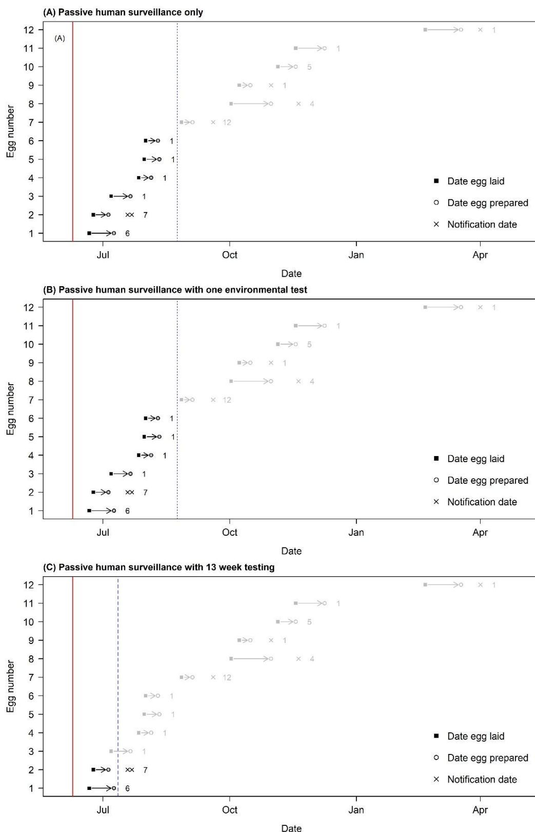
Figure 11: Small Farm with refrigeration iteration #1 – SE-positive eggs which caused illness with recall date: (A) PHS only, (B) PHS with one environmental test and (C) PHS with regular 13 week environmental tests. See Figure 10 for explanation of interpretation the figure contents
