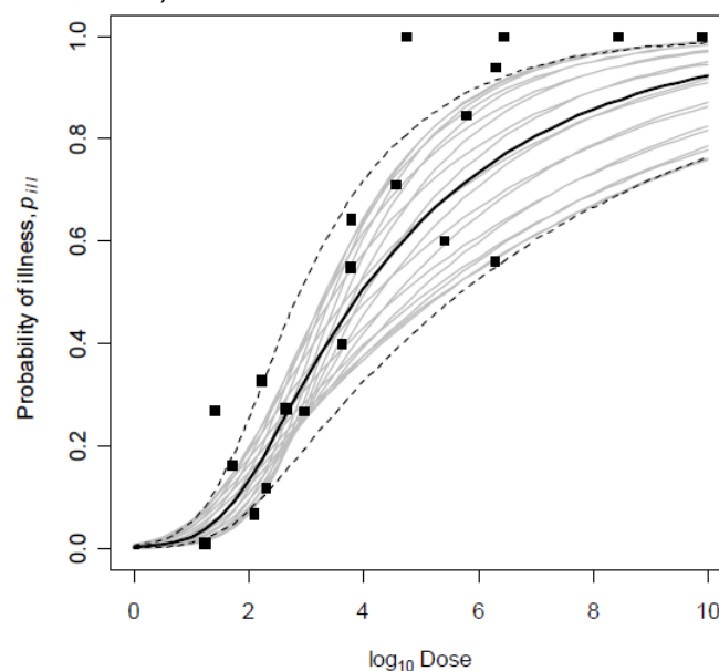
Figure 4: Uncertainty bounds for dose-response curves compared with expected value for the outbreak data (FAO/WHO, 2002; Thomas et al., 2006).
